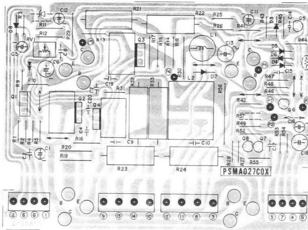
PSMA027COX MAIN AMP.
