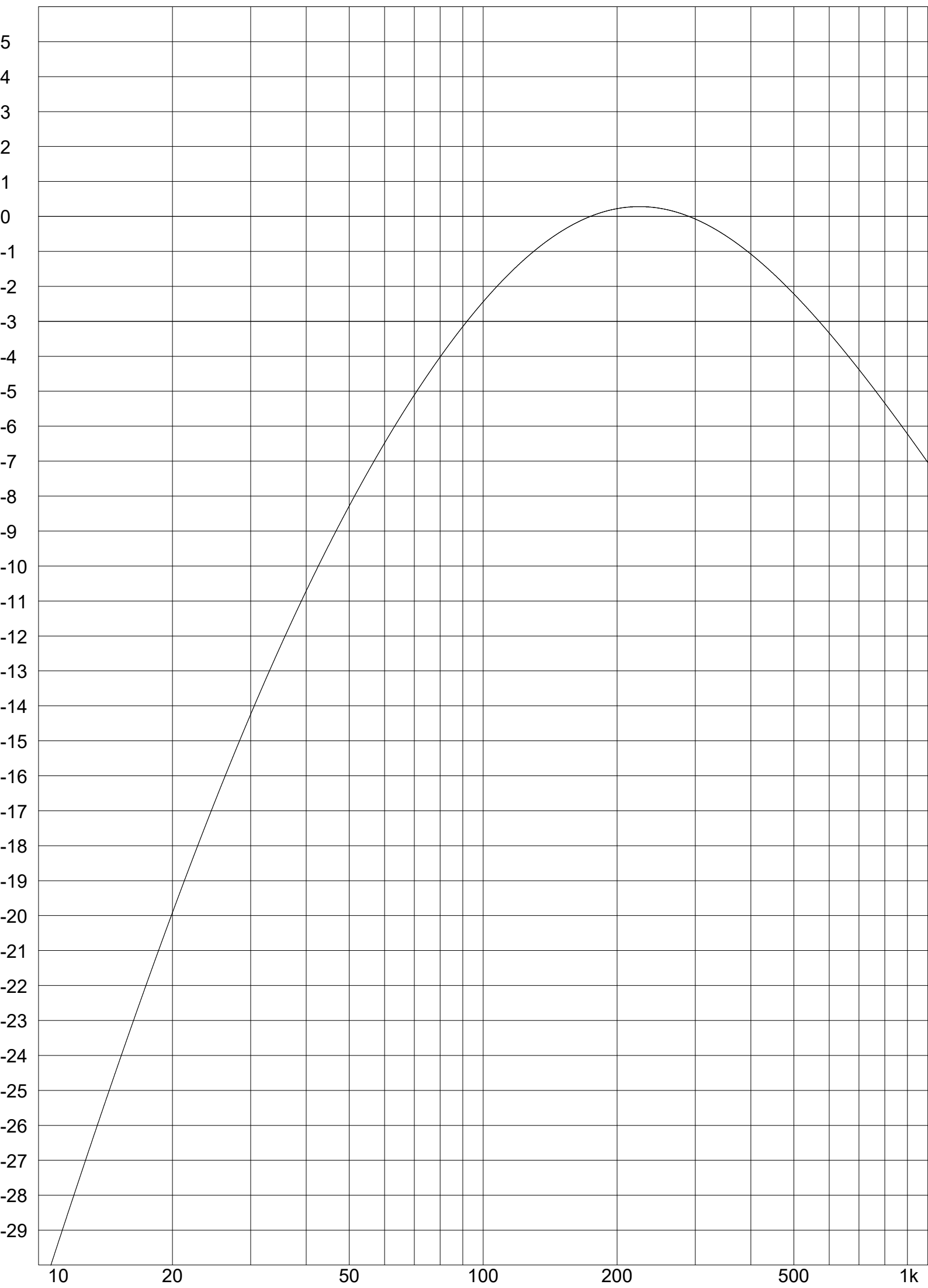
Transfer function magnitude [dB] - [1]closed : JBL 2226G
