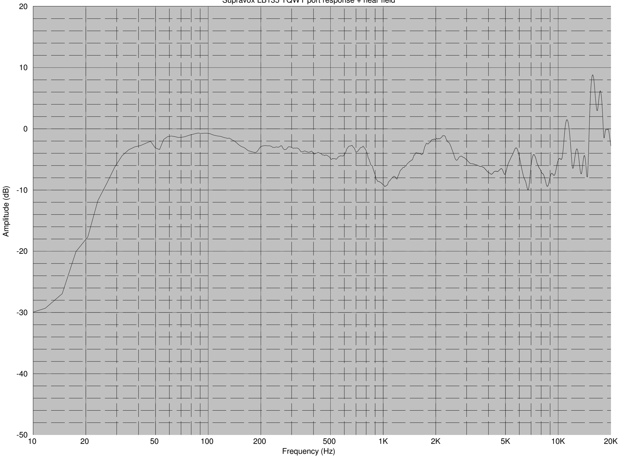
Supravox LB135 TQWT port response + near field
